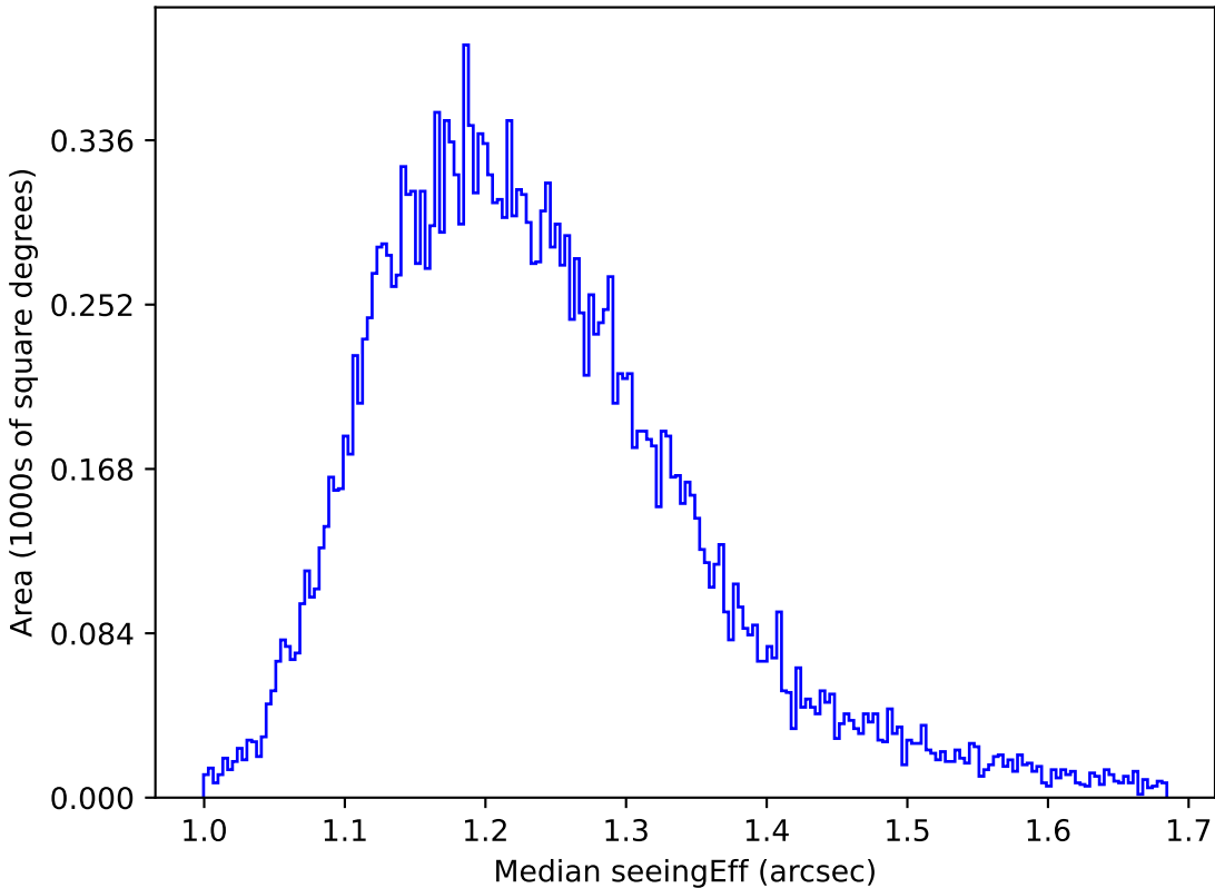
roll_pause_mjdp120_v3.4_10yrs All sky u band: Median seeingEff
