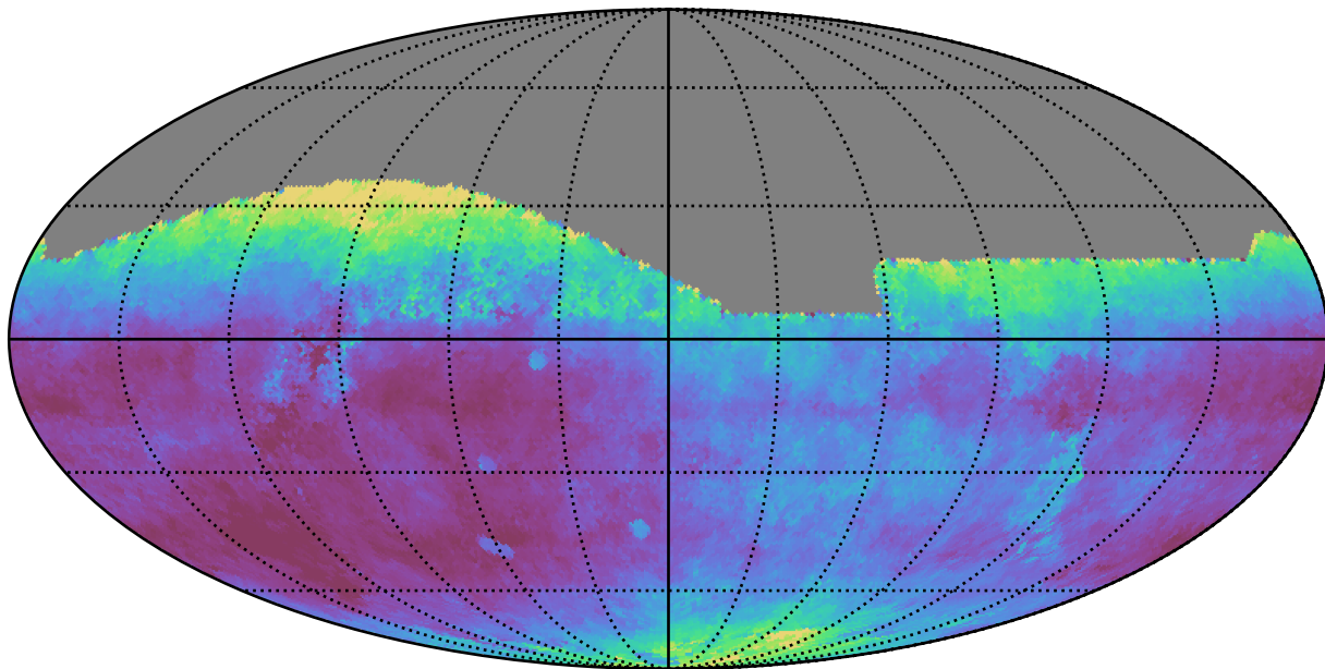
roll_pause_mjdp120_v3.4_10yrs All sky r band: Median seeingEff
