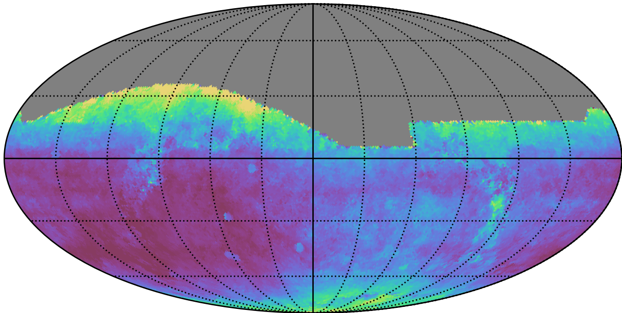
roll_pause_mjdp120_v3.4_10yrs All sky i band: Median seeingEff
