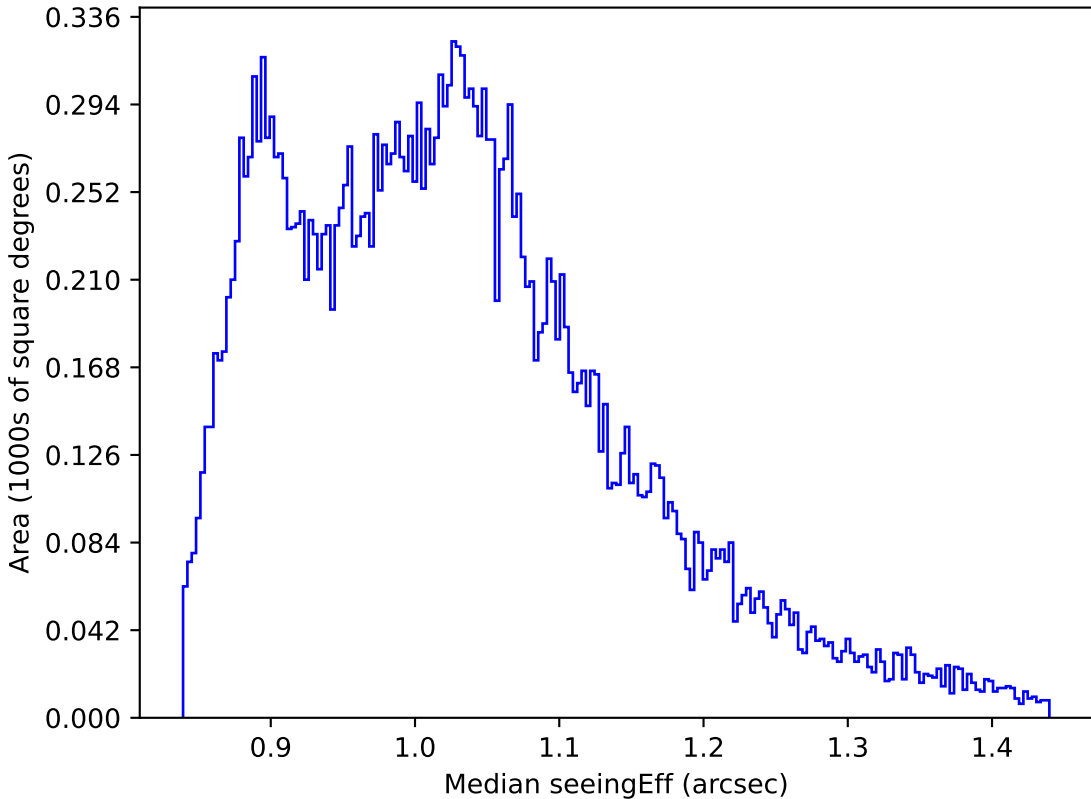
roll_pause_mjdp120_v3.4_10yrs All sky i band: Median seeingEff
