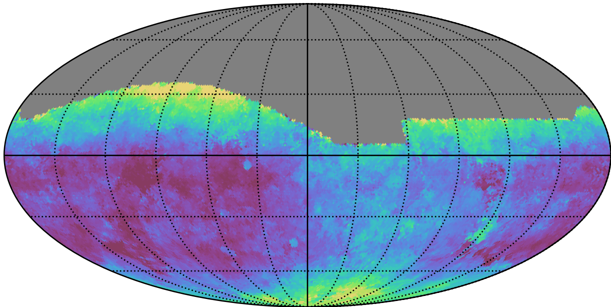
roll_pause_mjdp120_v3.4_10yrs All sky g band: Median seeingEff
