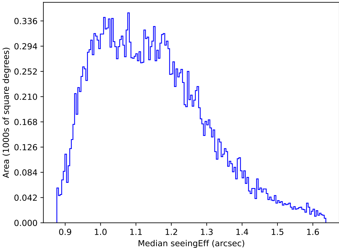
roll_pause_mjdp120_v3.4_10yrs All sky g band: Median seeingEff
