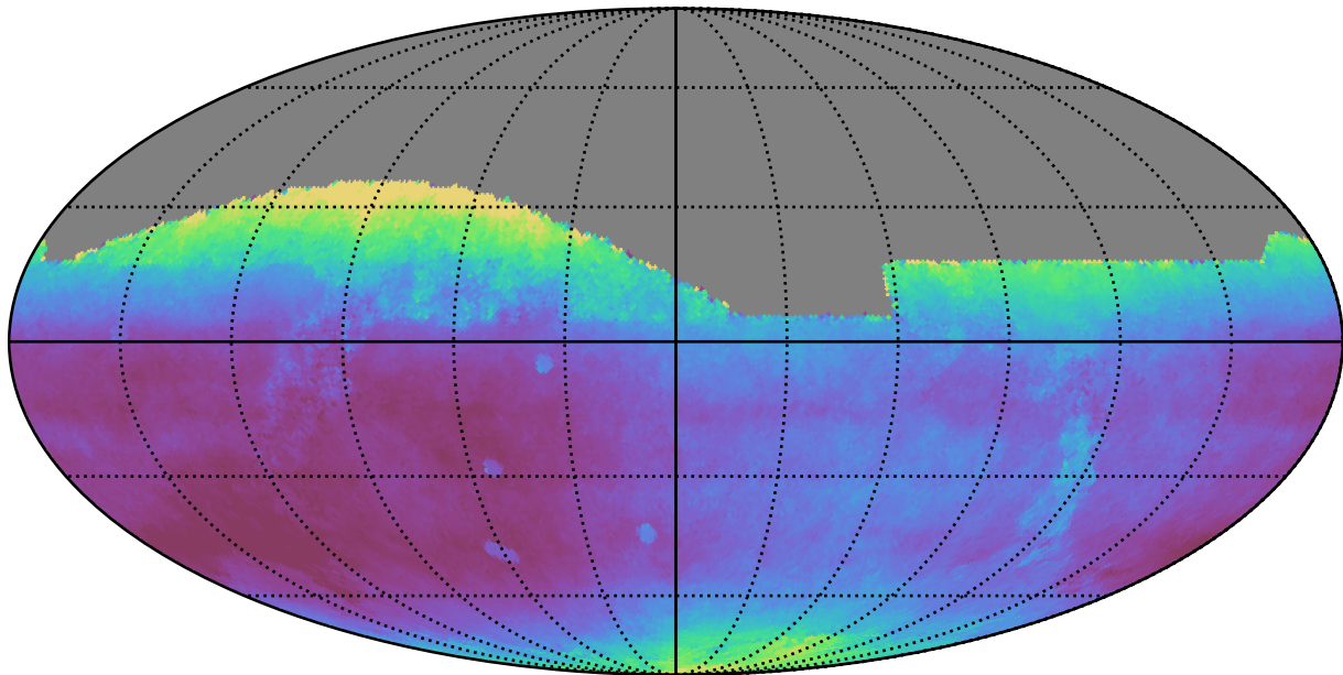
roll_pause_mjdp120_v3.4_10yrs All sky all bands: Median seeingEff
