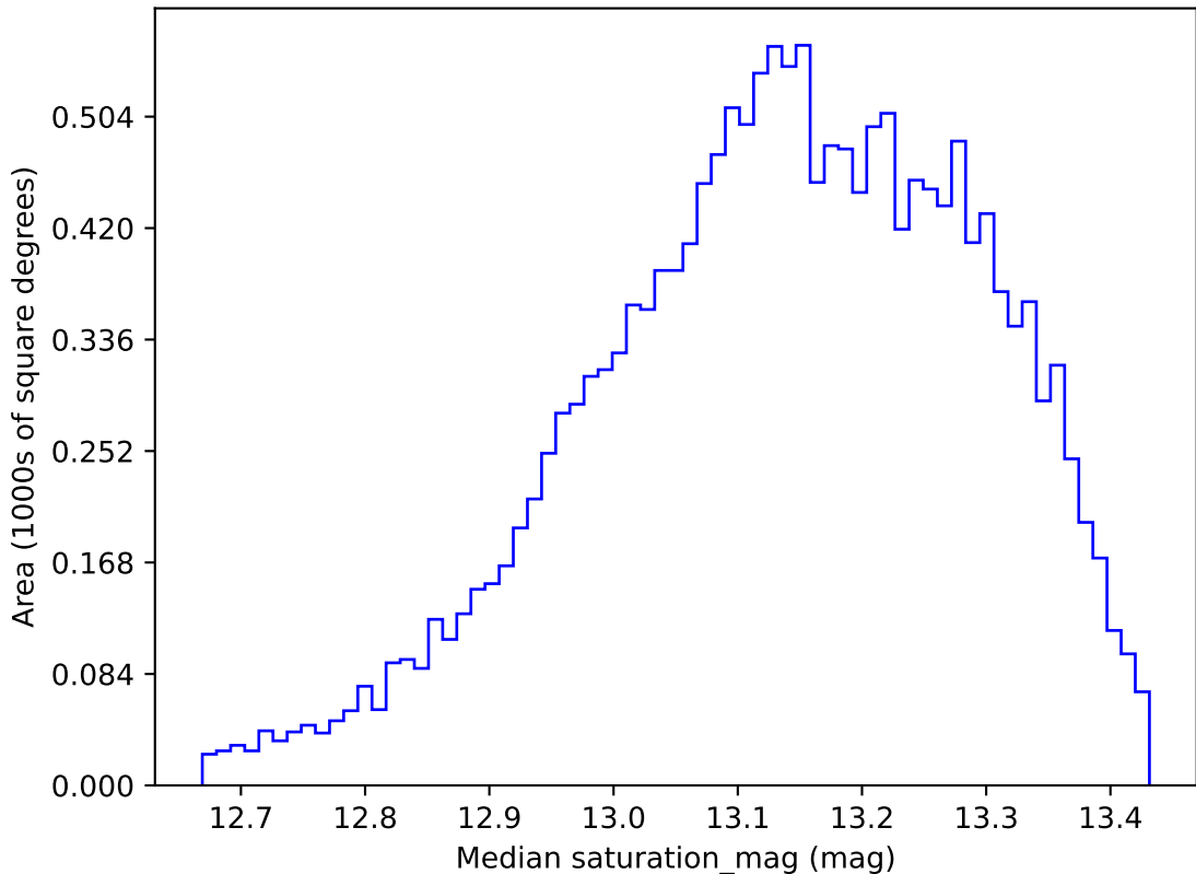
roll_pause_mjdp120_v3.4_10yrs WFD y band: Median saturation_mag
