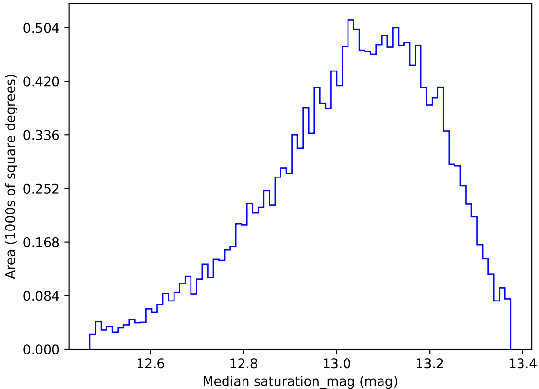
roll_pause_mjdp120_v3.4_10yrs WFD u band: Median saturation_mag
