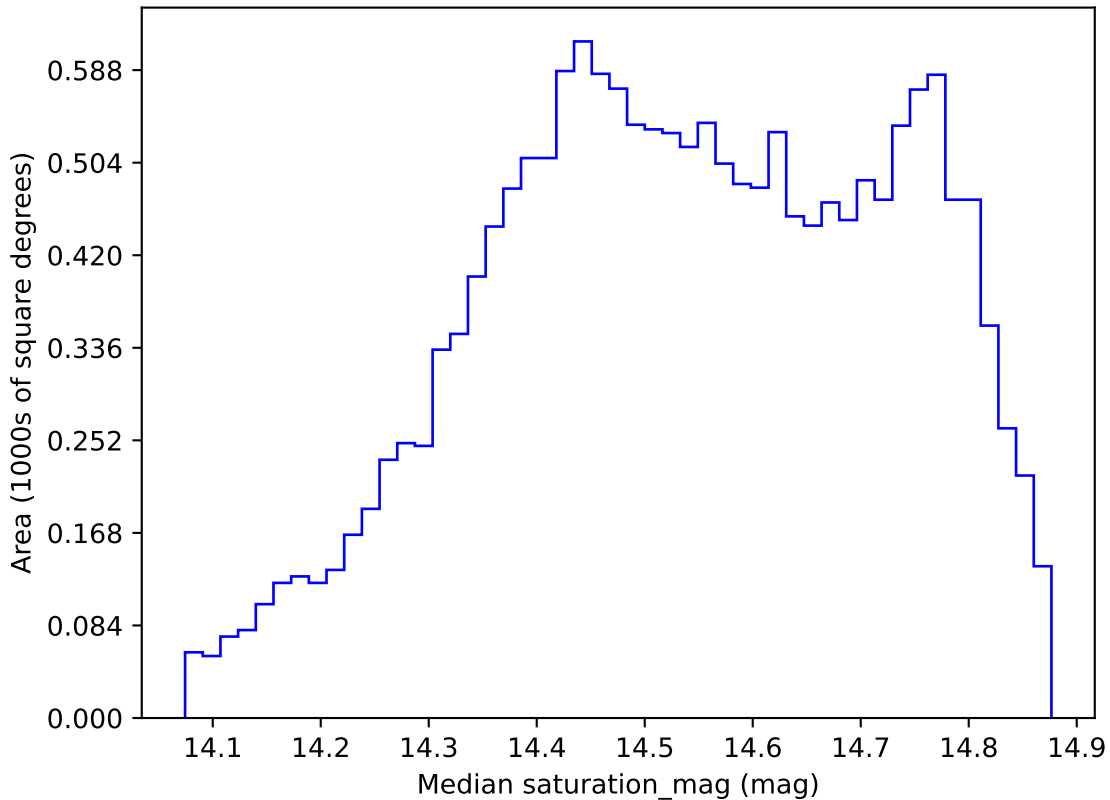
roll_pause_mjdp120_v3.4_10yrs WFD i band: Median saturation_mag
