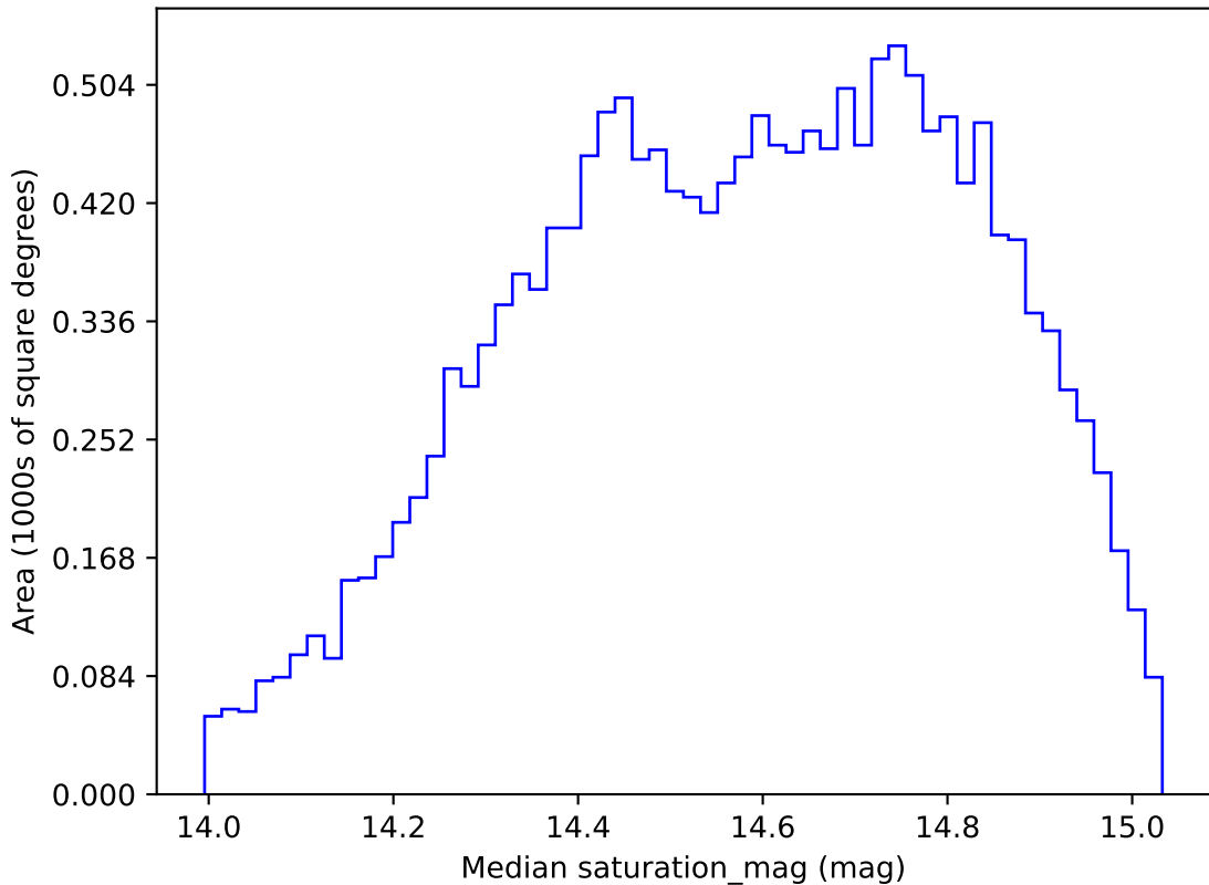
roll_pause_mjdp120_v3.4_10yrs WFD g band: Median saturation_mag
