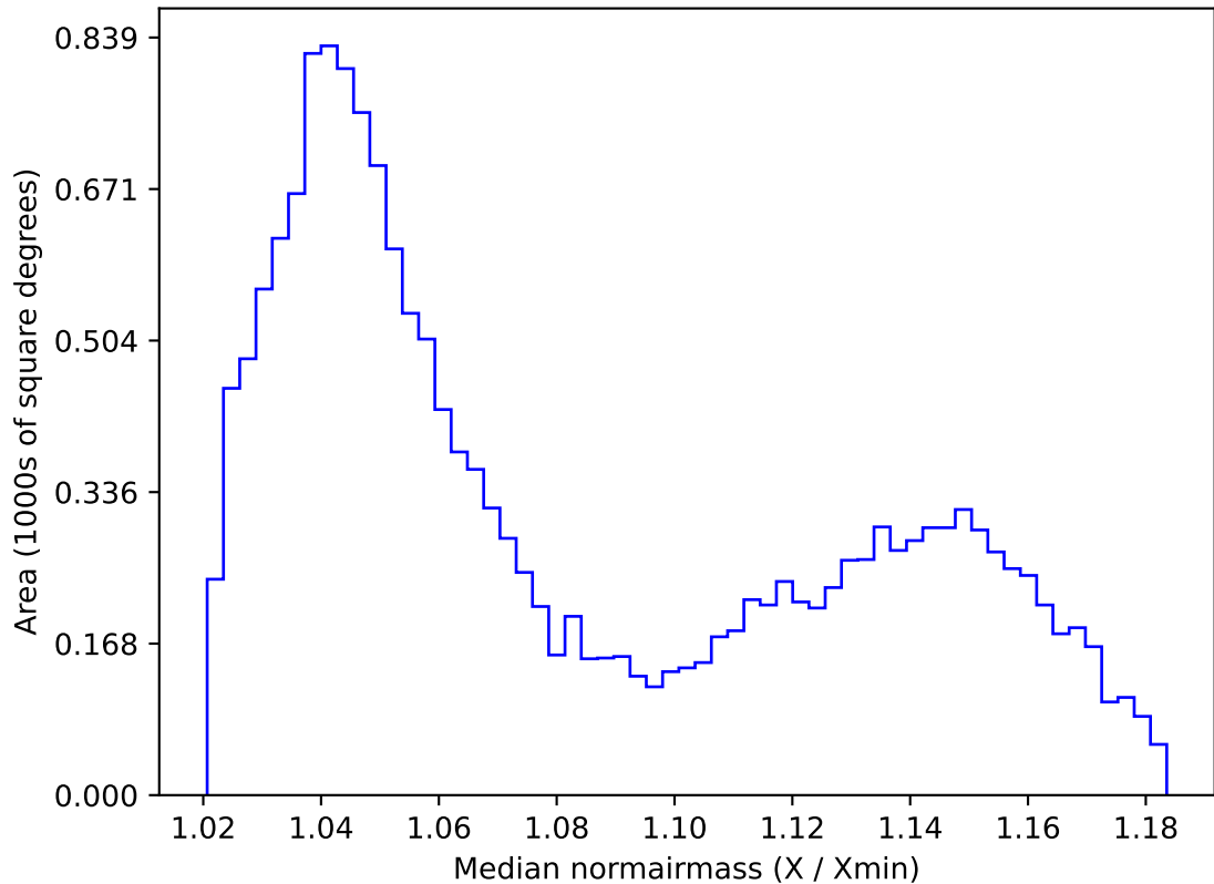
roll_pause_mjdp120_v3.4_10yrs WFD z band: Median normairmass
