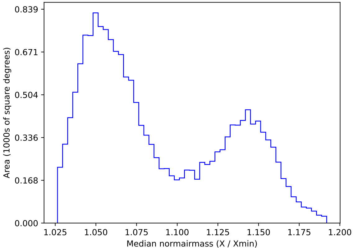
roll_pause_mjdp120_v3.4_10yrs WFD y band: Median normairmass
