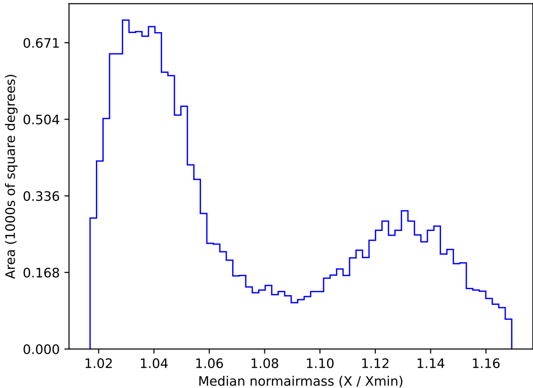
roll_pause_mjdp120_v3.4_10yrs WFD i band: Median normairmass
