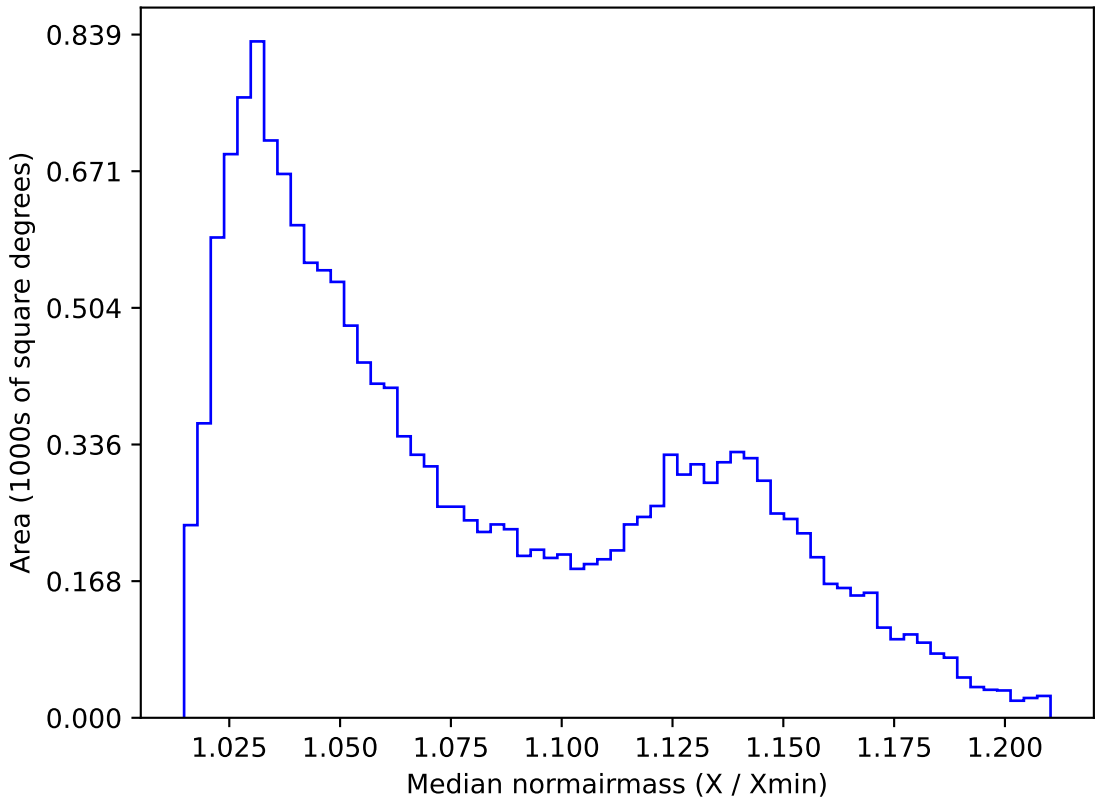
roll_pause_mjdp120_v3.4_10yrs WFD g band: Median normairmass
