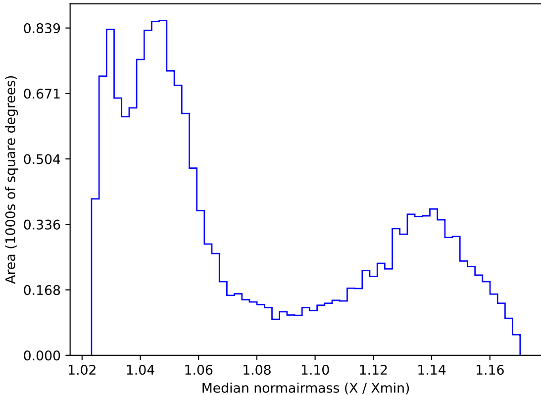
roll_pause_mjdp120_v3.4_10yrs WFD all bands: Median normairmass
