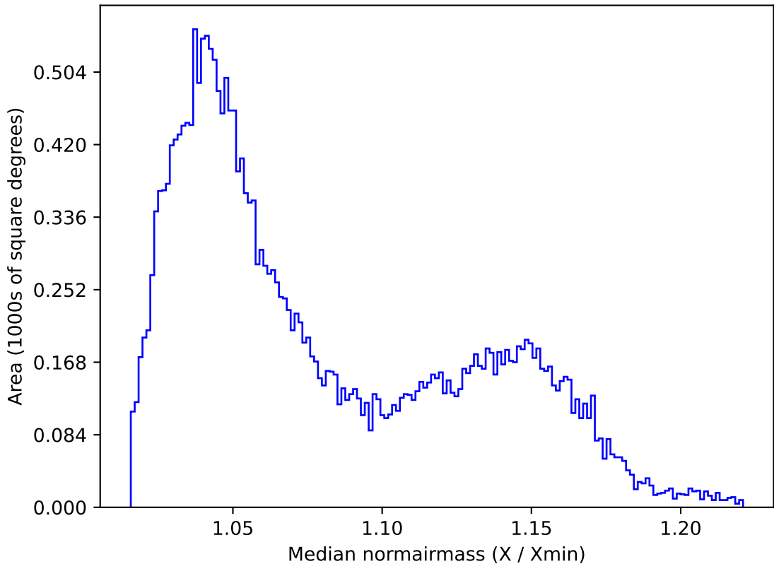
roll_pause_mjdp120_v3.4_10yrs All sky z band: Median normairmass
