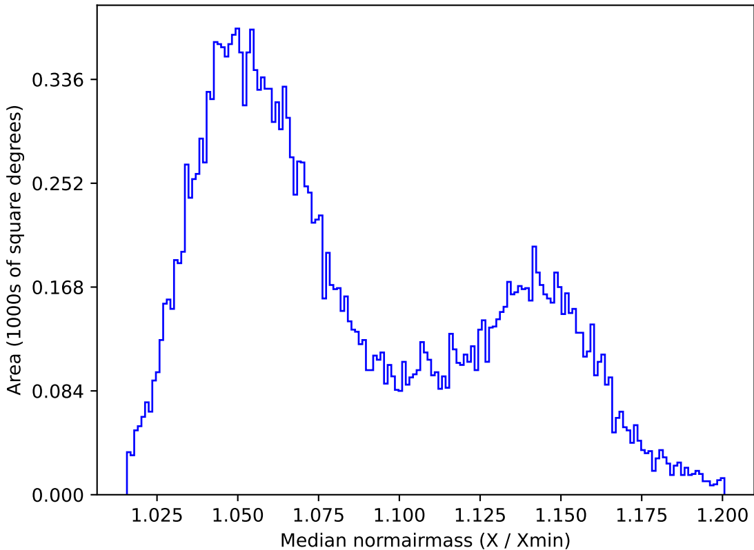
roll_pause_mjdp120_v3.4_10yrs All sky y band: Median normairmass
