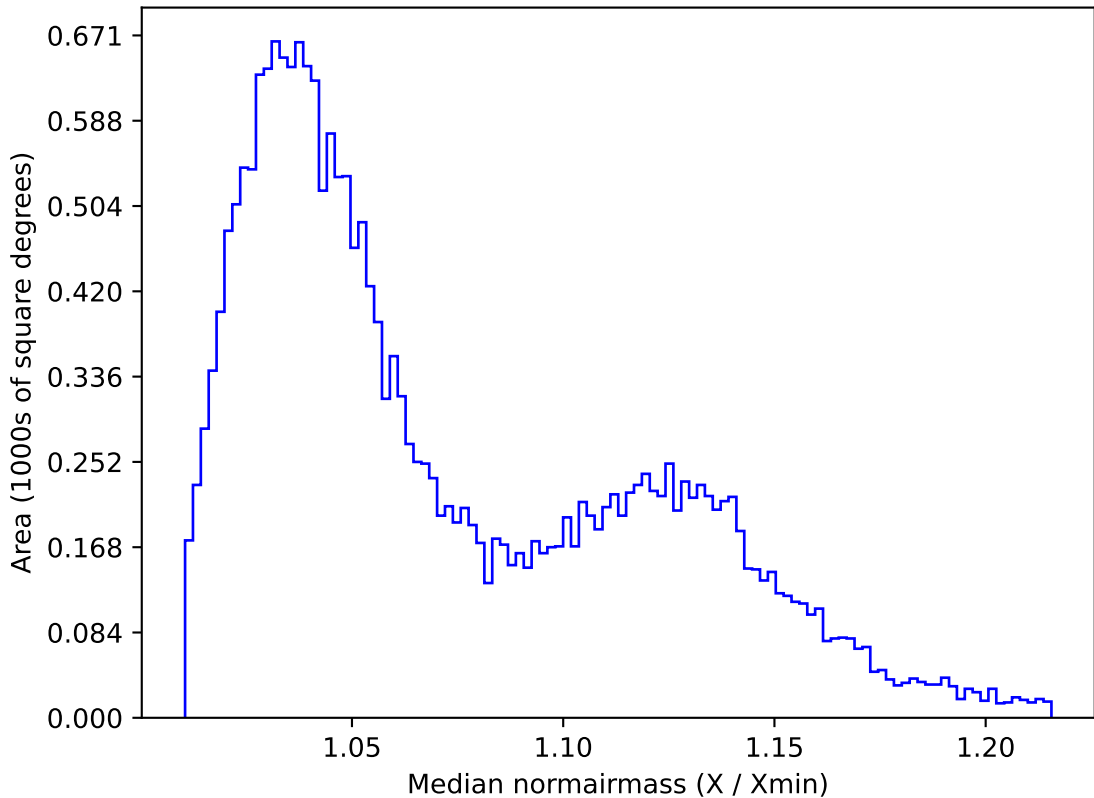
roll_pause_mjdp120_v3.4_10yrs All sky u band: Median normairmass
