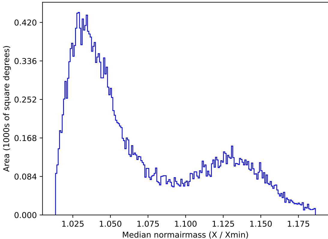
roll_pause_mjdp120_v3.4_10yrs All sky r band: Median normairmass
