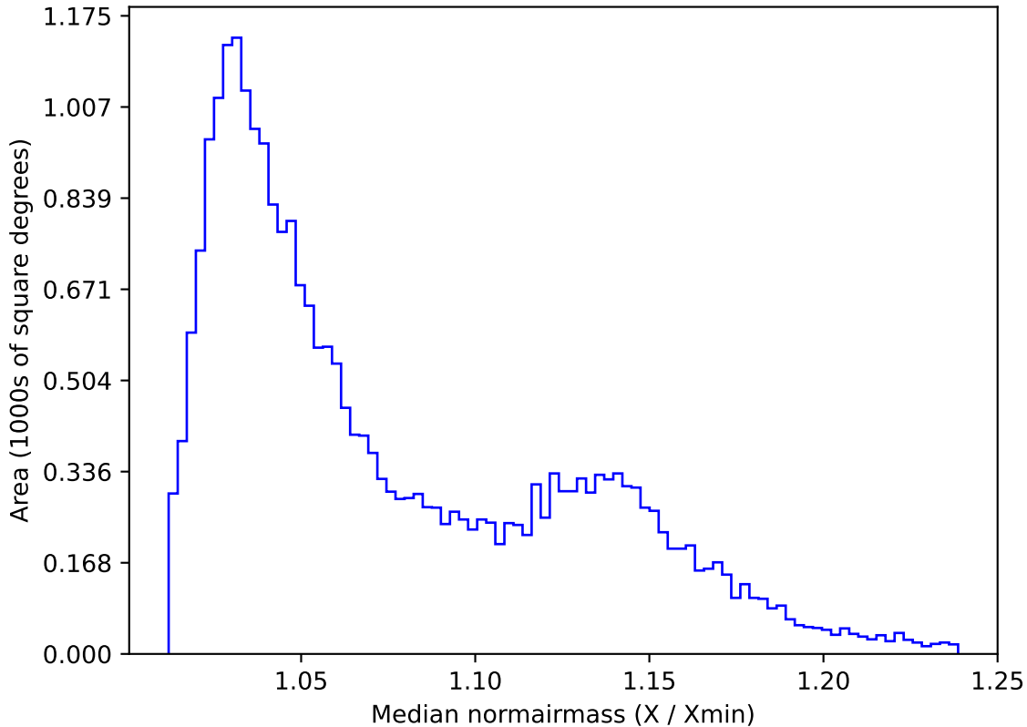
roll_pause_mjdp120_v3.4_10yrs All sky g band: Median normairmass
