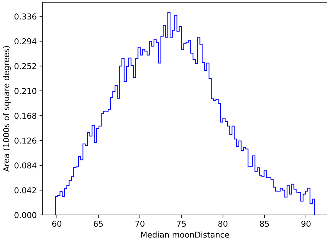
roll_pause_mjdp120_v3.4_10yrs WFD z band: Median moonDistance
