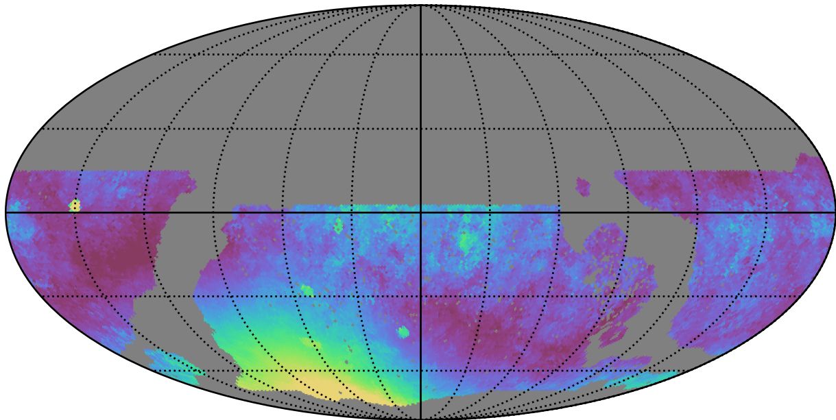
roll_pause_mjdp120_v3.4_10yrs WFD y band: Median moonDistance
