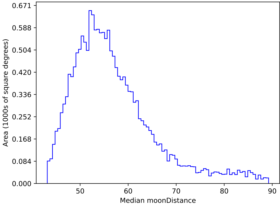
roll_pause_mjdp120_v3.4_10yrs WFD y band: Median moonDistance
