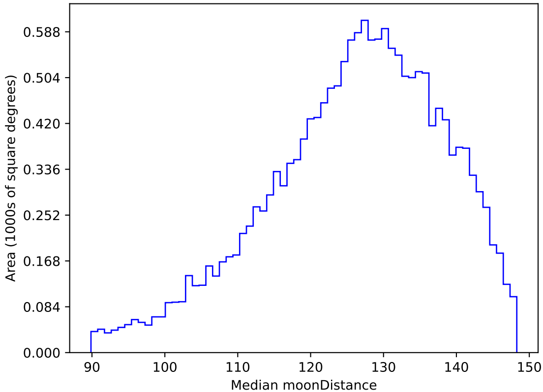
roll_pause_mjdp120_v3.4_10yrs WFD u band: Median moonDistance
