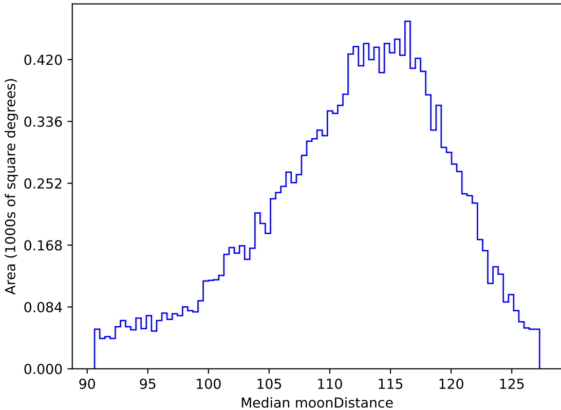
roll_pause_mjdp120_v3.4_10yrs WFD r band: Median moonDistance
