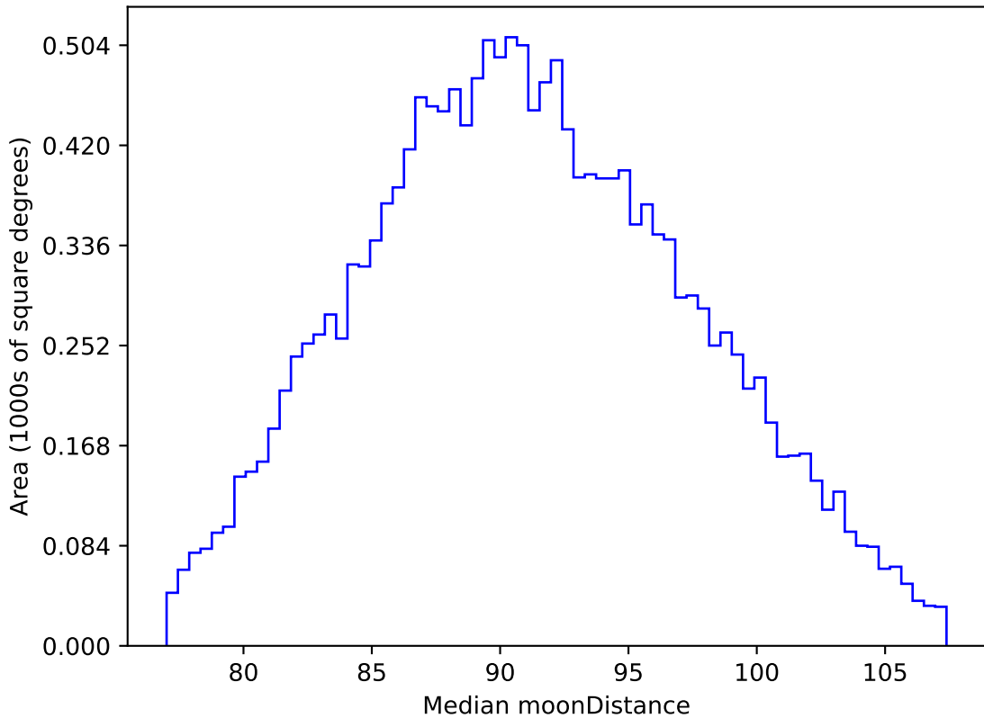
roll_pause_mjdp120_v3.4_10yrs WFD i band: Median moonDistance
