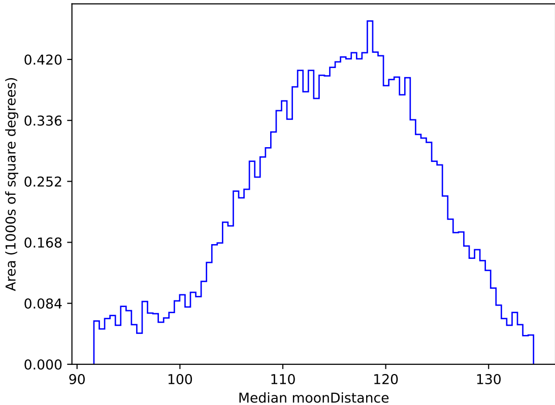
roll_pause_mjdp120_v3.4_10yrs WFD g band: Median moonDistance
