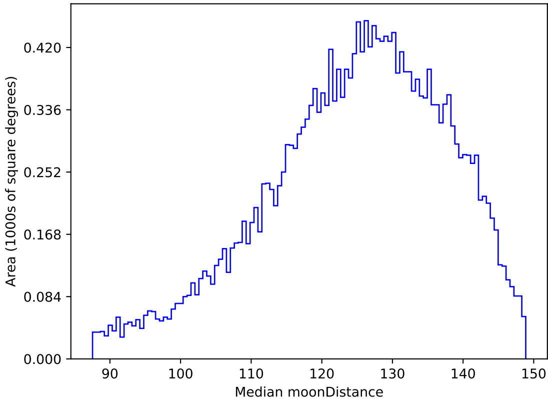
roll_pause_mjdp120_v3.4_10yrs All sky u band: Median moonDistance
