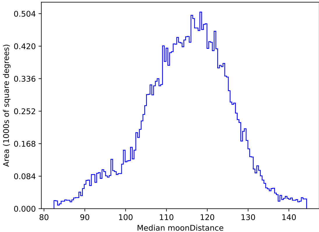
roll_pause_mjdp120_v3.4_10yrs All sky g band: Median moonDistance
