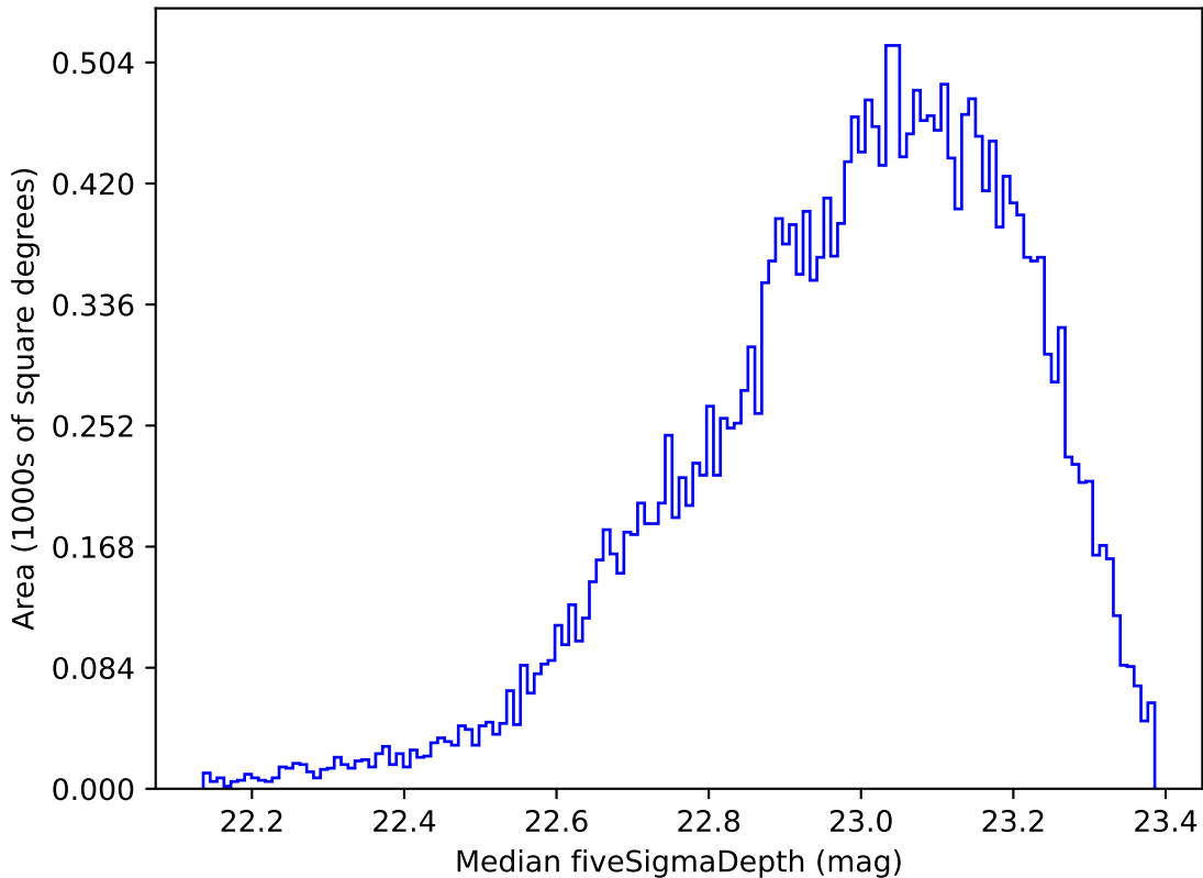
roll_pause_mjdp120_v3.4_10yrs Yr 1 z band: Median fiveSigmaDepth
