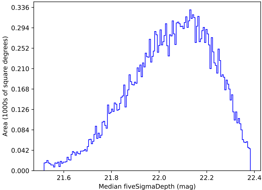
roll_pause_mjdp120_v3.4_10yrs Yr 1 y band: Median fiveSigmaDepth
