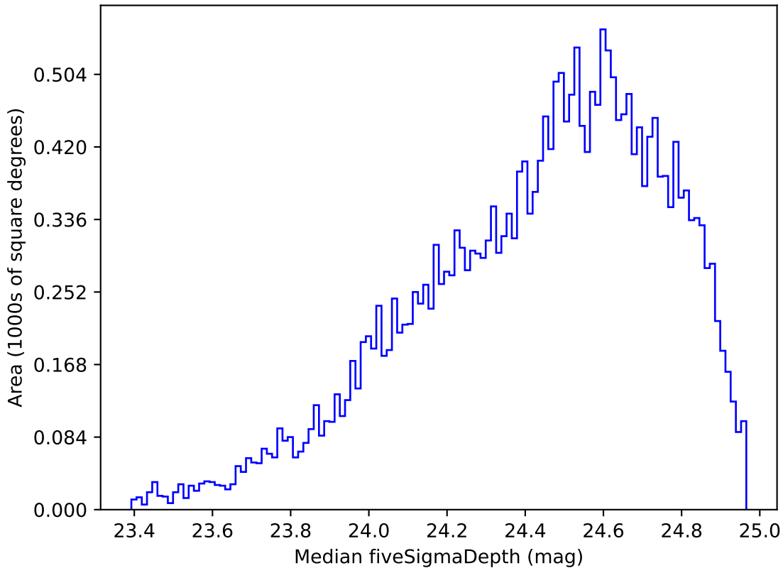
roll_pause_mjdp120_v3.4_10yrs Yr 1 g band: Median fiveSigmaDepth
