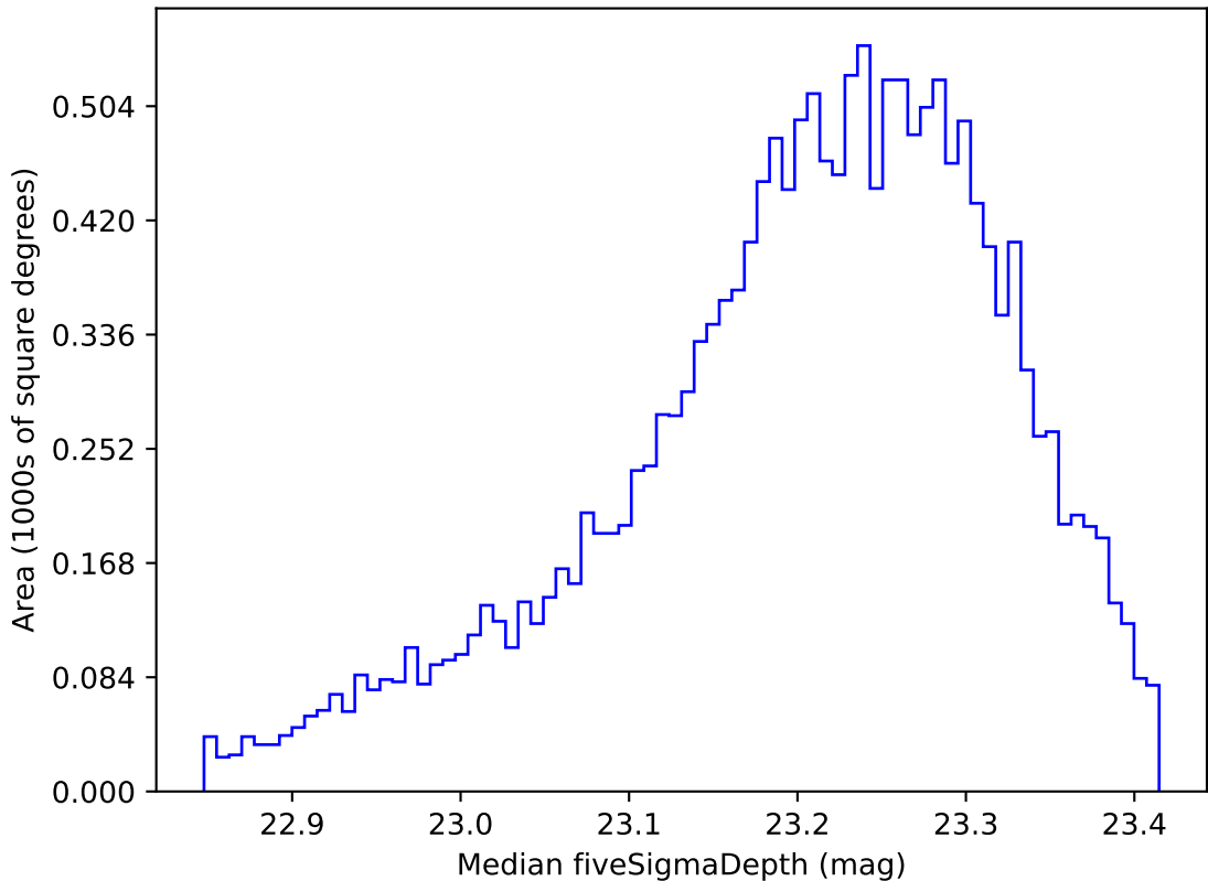
roll_pause_mjdp120_v3.4_10yrs WFD u band: Median fiveSigmaDepth
