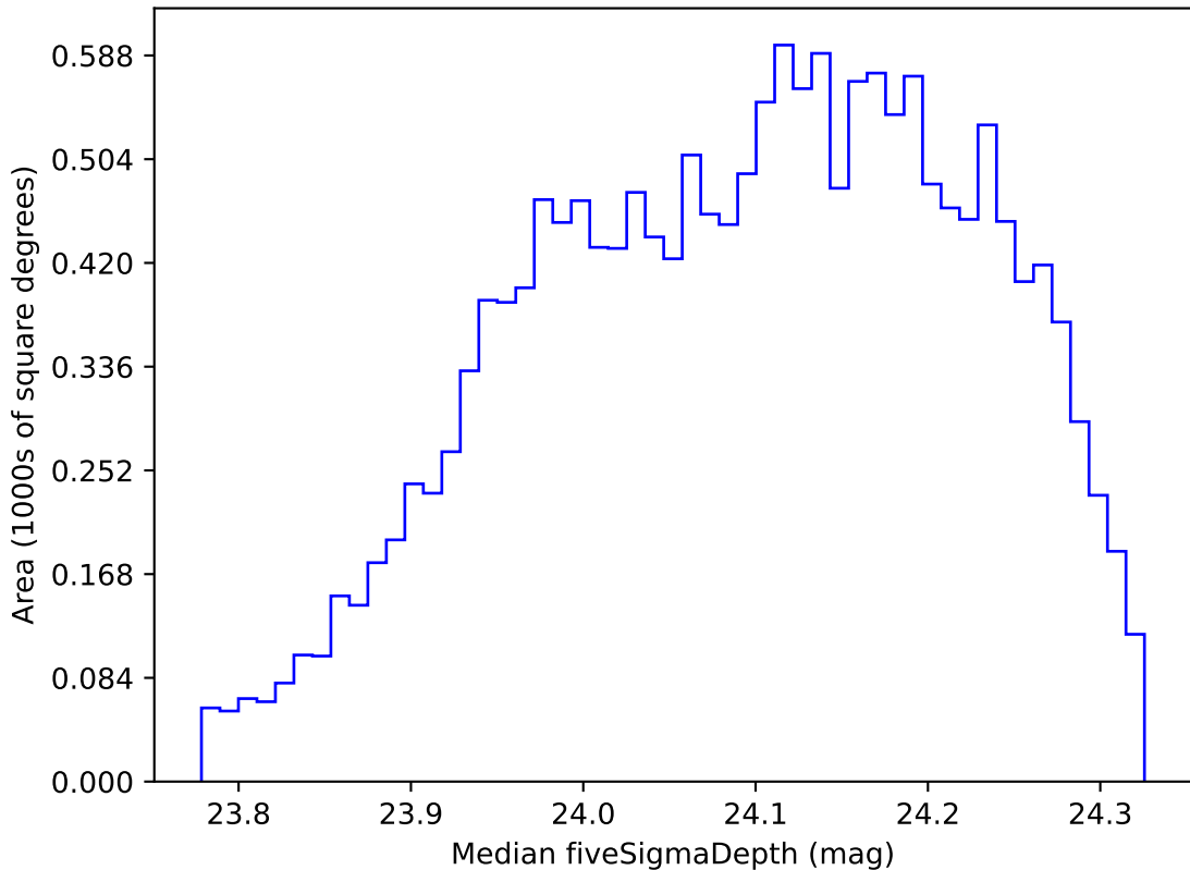
roll_pause_mjdp120_v3.4_10yrs WFD r band: Median fiveSigmaDepth
