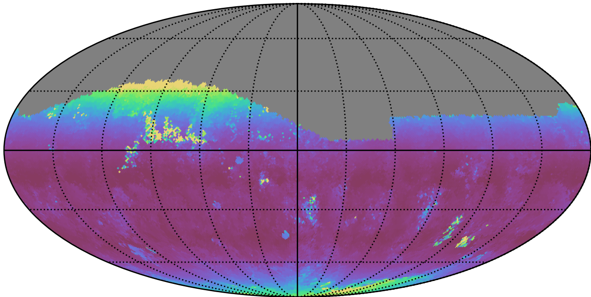
roll_pause_mjdp120_v3.4_10yrs Yr 1 z band: Median airmass
