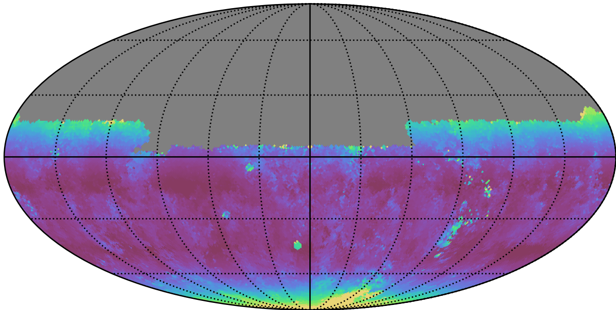
roll_pause_mjdp120_v3.4_10yrs Yr 1 y band: Median airmass
