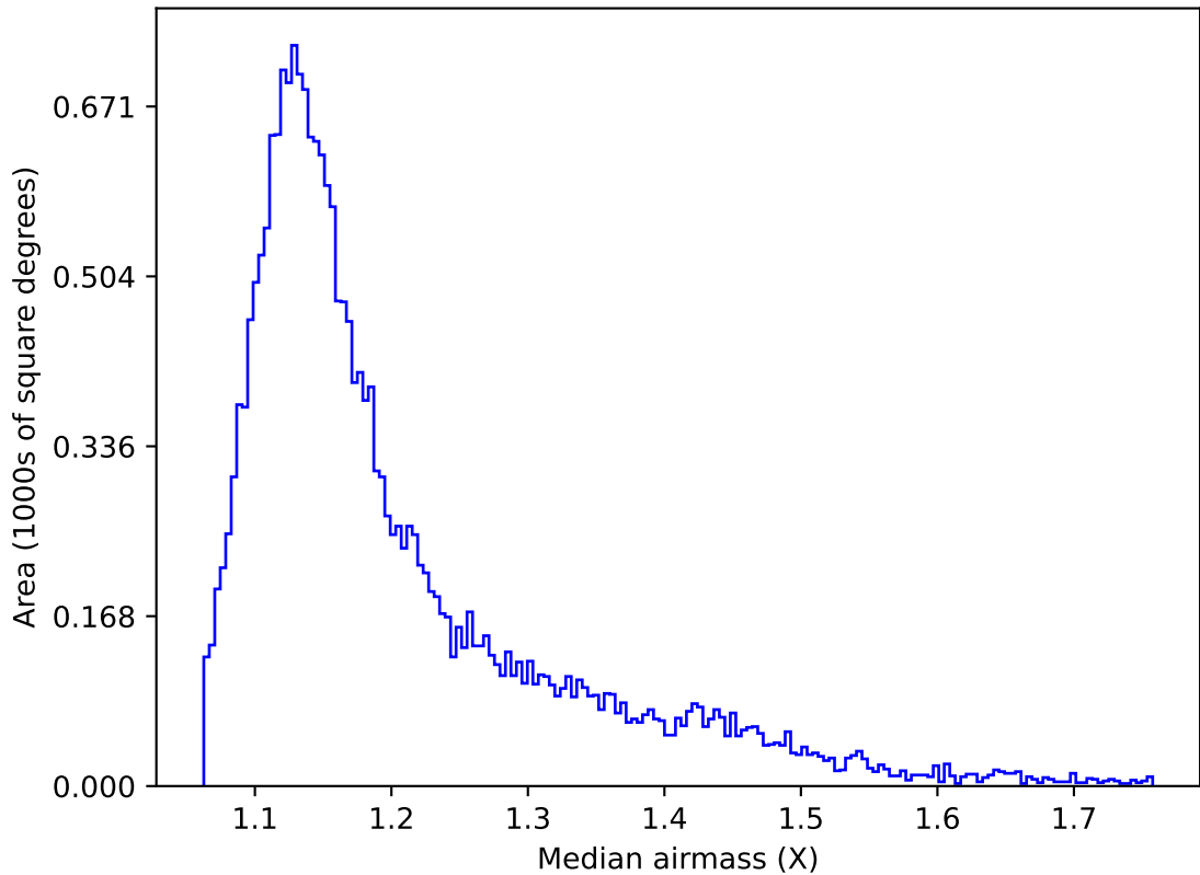
roll_pause_mjdp120_v3.4_10yrs Yr 1 y band: Median airmass
