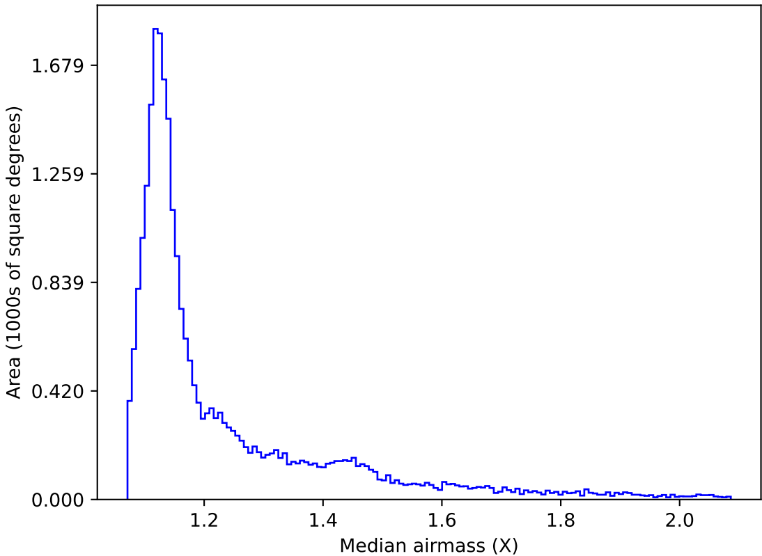
roll_pause_mjdp120_v3.4_10yrs Yr 1 all bands: Median airmass
