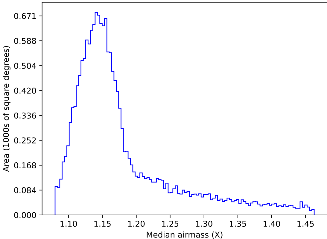
roll_pause_mjdp120_v3.4_10yrs WFD z band: Median airmass
