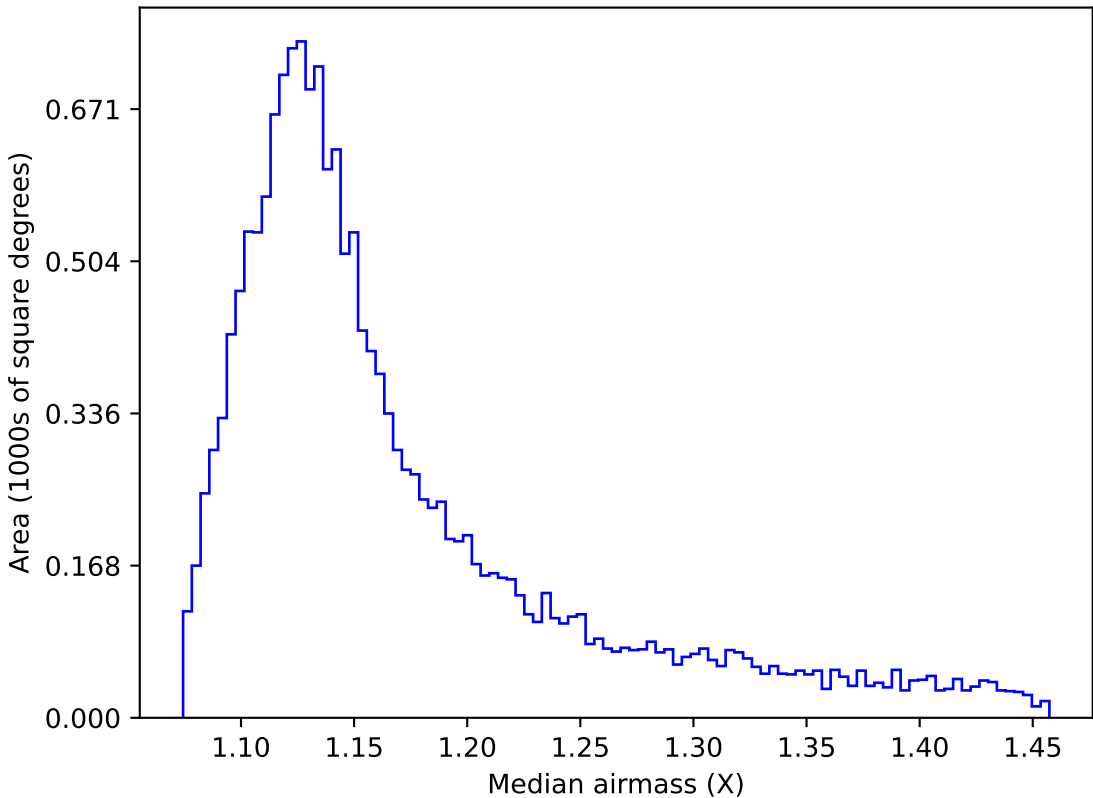
roll_pause_mjdp120_v3.4_10yrs WFD u band: Median airmass
