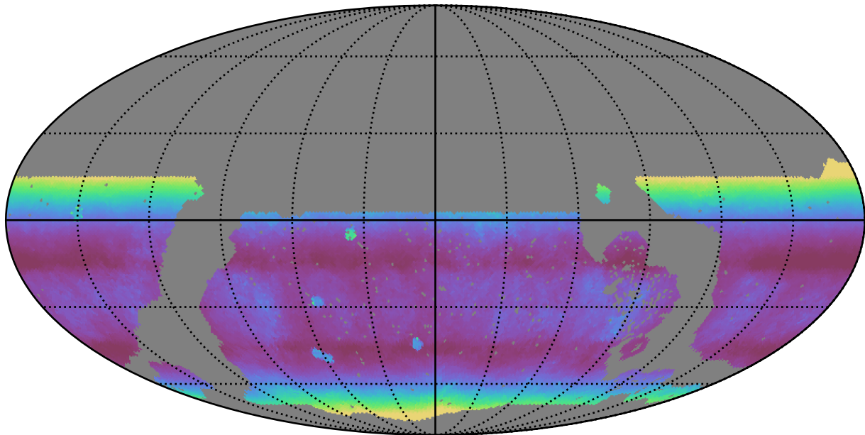
roll_pause_mjdp120_v3.4_10yrs WFD r band: Median airmass
