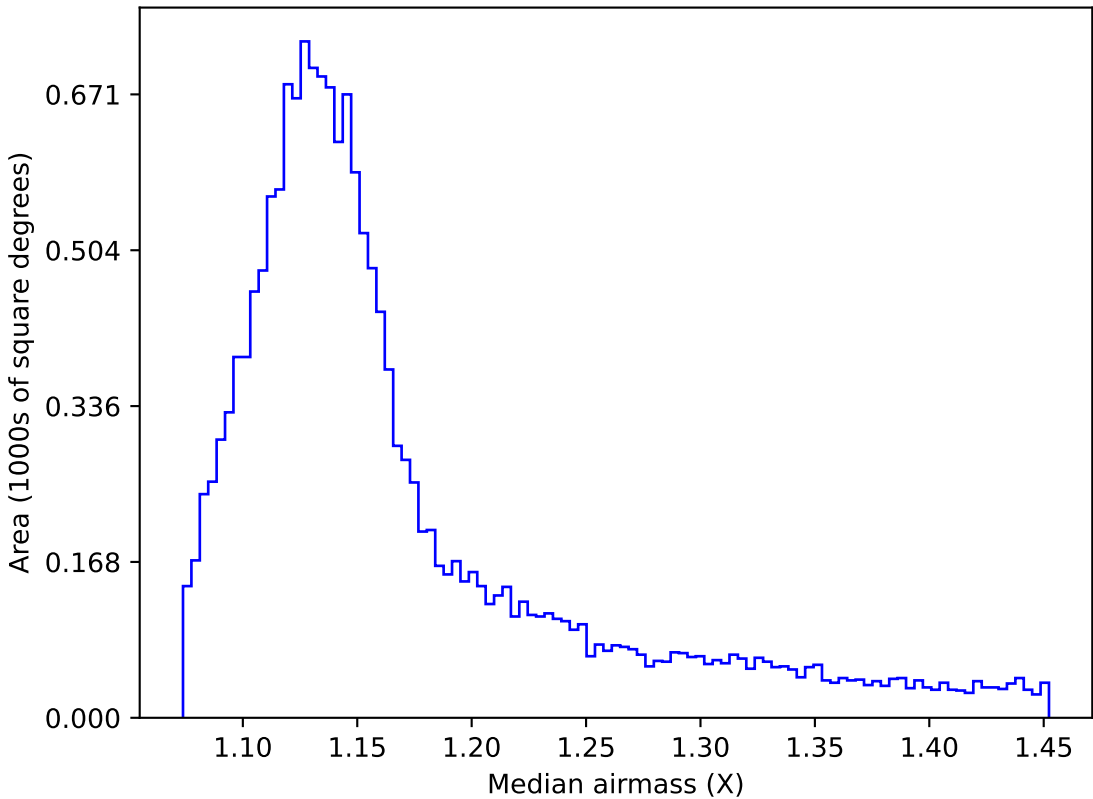
roll_pause_mjdp120_v3.4_10yrs WFD r band: Median airmass
