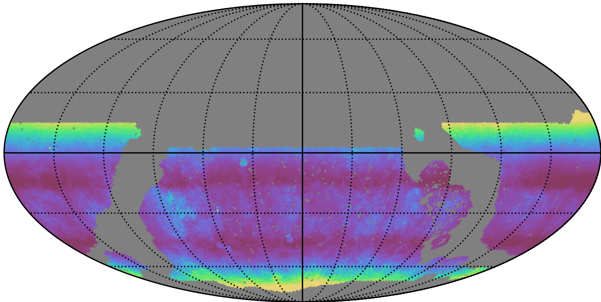
roll_pause_mjdp120_v3.4_10yrs WFD g band: Median airmass
