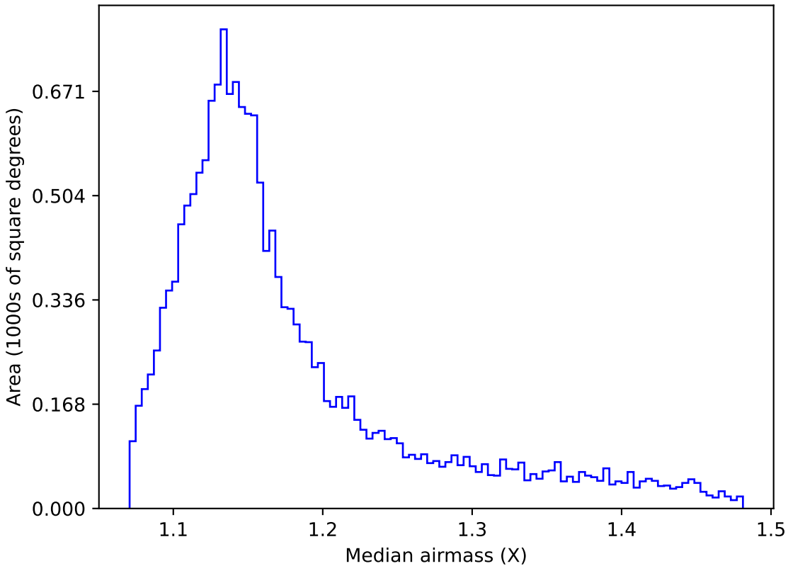
roll_pause_mjdp120_v3.4_10yrs WFD g band: Median airmass
