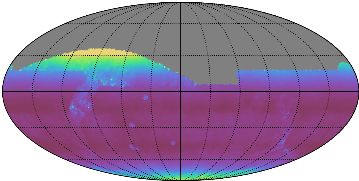
roll_pause_mjdp120_v3.4_10yrs All sky z band: Median airmass
