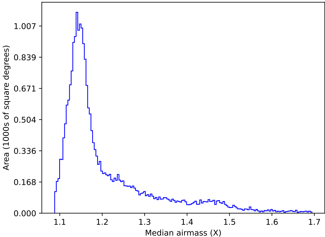
roll_pause_mjdp120_v3.4_10yrs All sky y band: Median airmass
