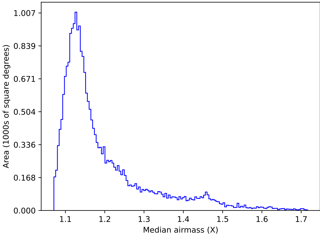
roll_pause_mjdp120_v3.4_10yrs All sky u band: Median airmass
