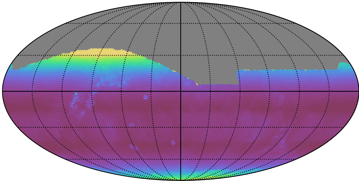
roll_pause_mjdp120_v3.4_10yrs All sky r band: Median airmass
