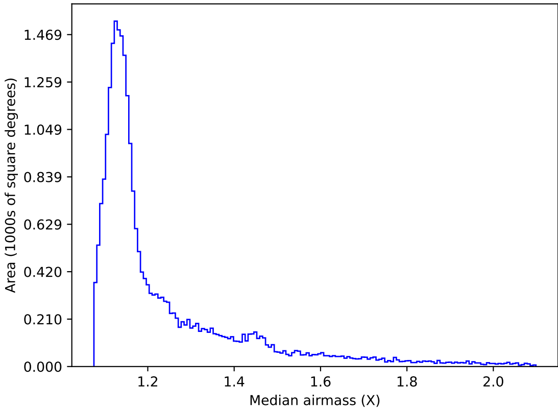
roll_pause_mjdp120_v3.4_10yrs All sky r band: Median airmass
